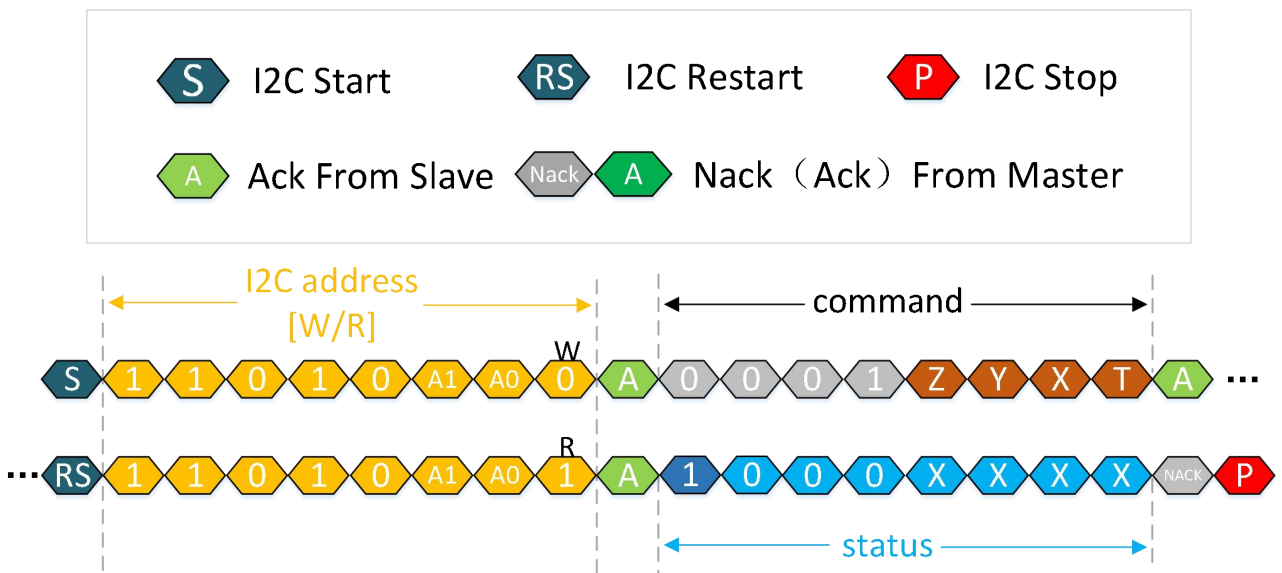
Figure 8-2. Continuous Sensing Mode I2C Communication Diagram
