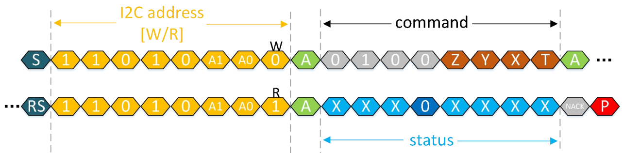
Figure 11-4. Data Read Frame TXYZ I2C Communication Diagram
