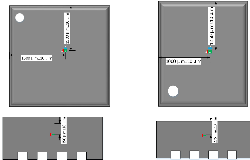
Figure 7-2. The relative position of sensitive area in the QFN3x3 16-Pin package
