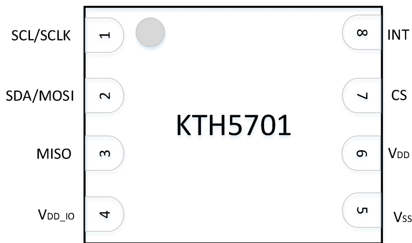
figure5-2. DFN2x2.5 8-Pin Top view
