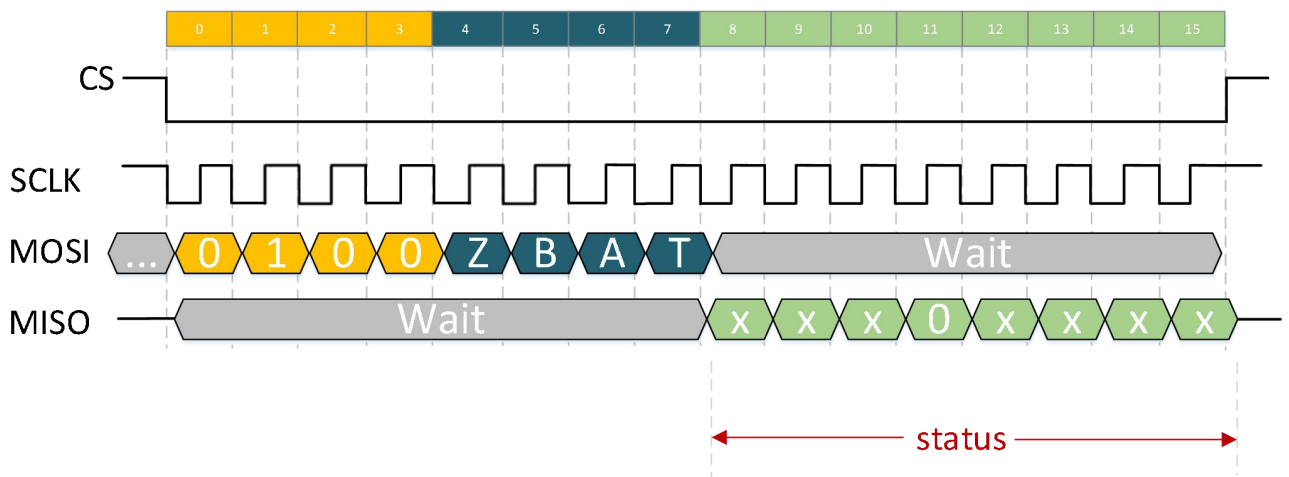
Figure 11-9. TABZ Data Read Back SPI Communication Diagram
