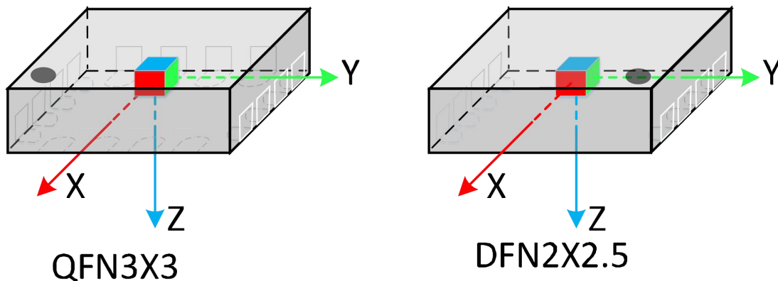
Figure 7-1. Schematic diagram of the sensitive direction of each axis producing the ADC positive output
