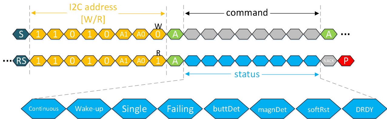
Figure 10-2. Operating Status I2C Description
